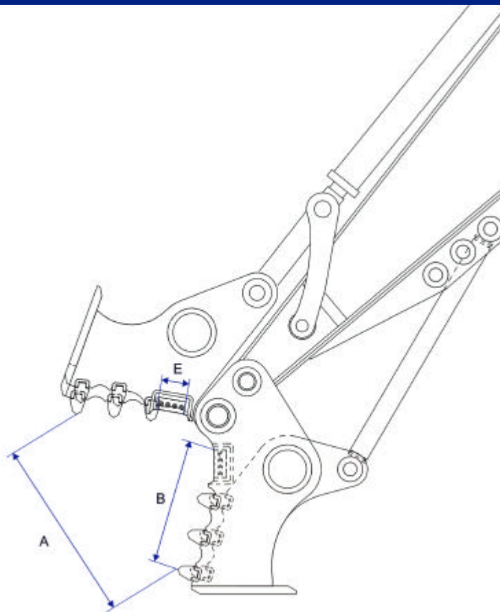
Upper (Moveable) Jaw
